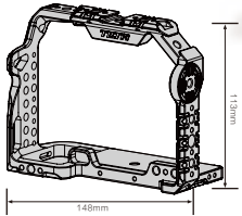
TA-T23-FCC-B FULL CAMERA CAGE FOR SONY A1
