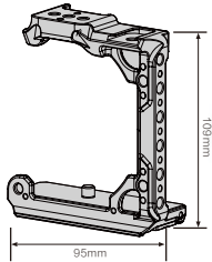
TA-T23-HCC-B HALF CAMERA CAGE FOR SONY A1
