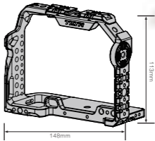
TA-T23-FCC-B FULL CAMERA CAGE FOR SONY A1
